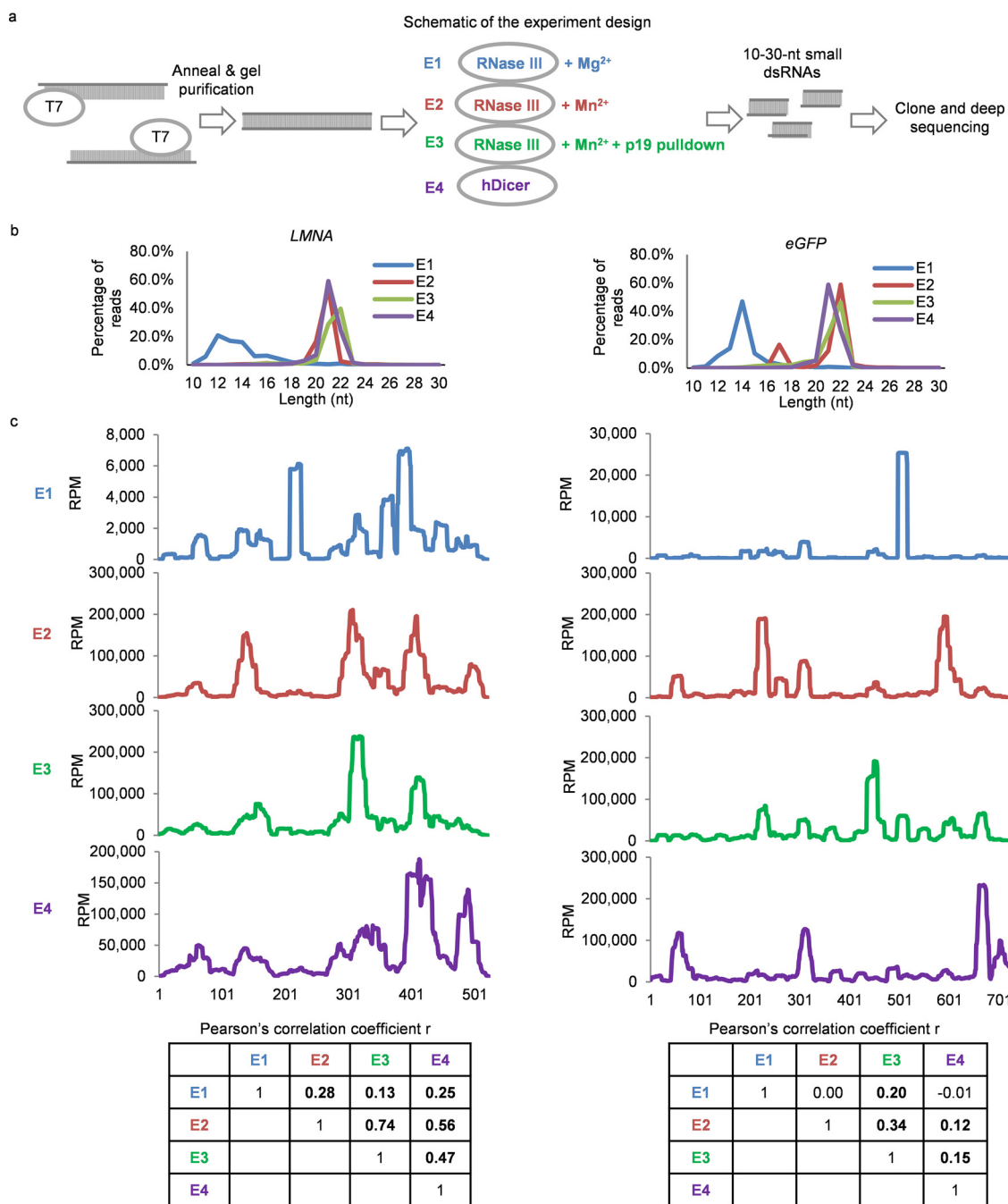
FIG 2 Hot spots of p19-captured dsRNAs are caused by RNase III. (a) Schematic of experiment design. (b) Length distribution of small RNA deep-sequencing data. (c) Deep-sequencing reads (combining sense and antisense reads) plotted along a 523-bp fragment of LMNA (left) and a 720-bp fragment of eGFP . RPM, reads per million. (Bottom) Pairwise correlation coefficient table calculated using small RNA sequence profiles. In boldface are those correlations with a P value of <0.05 .
