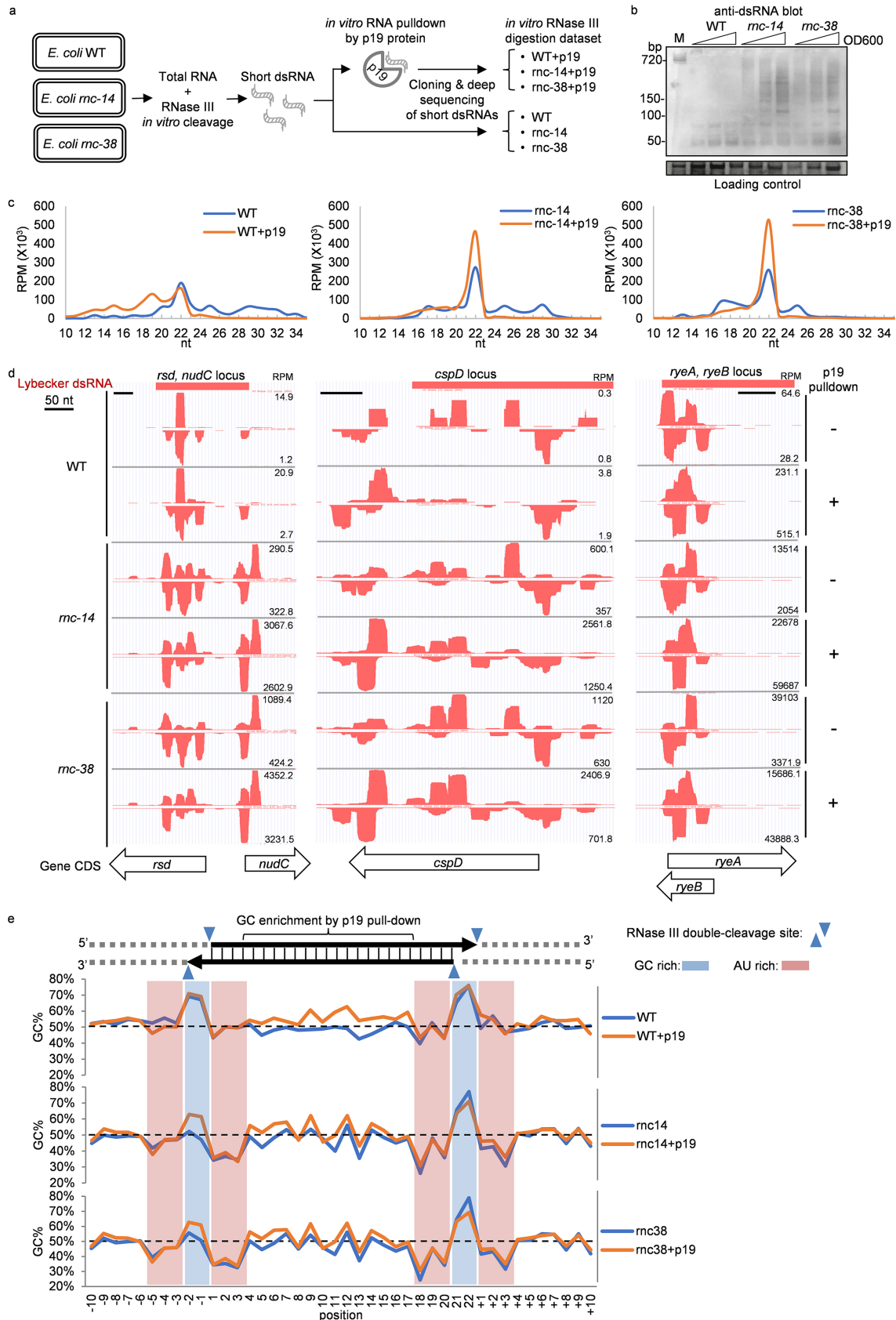
FIG 3 Sequence biases of RNase III p19 pulldown. (a) Schematic of in vitro RNase III digestion experiment on E. coli total RNA followed by p19 pulldown. (b) dsRNA immunoblot of E. coli total RNA probed with J2 anti-dsRNA antibody. The loading control is a major RNA (Continued on next page)
