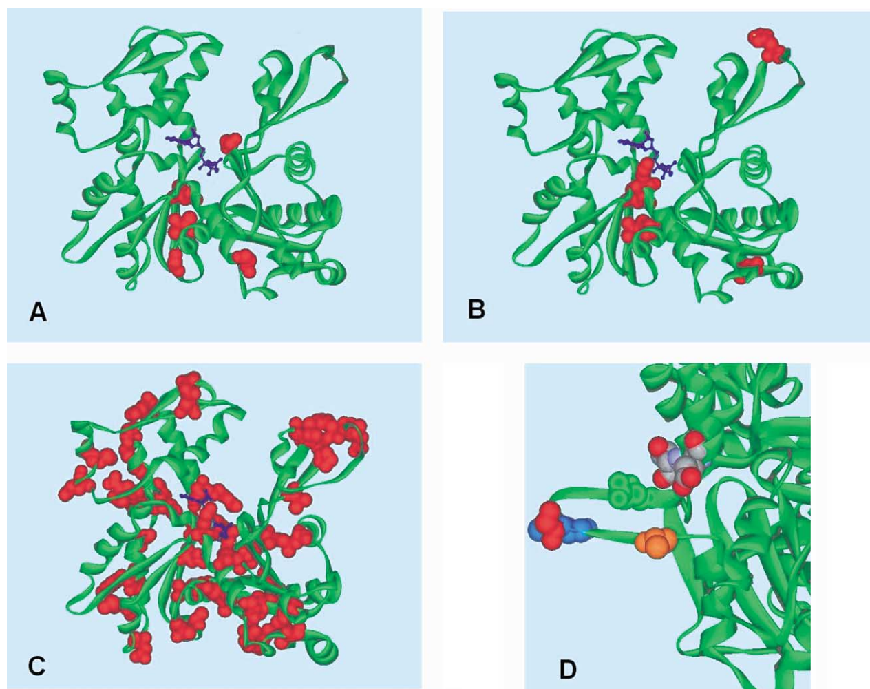
Fig. 4. Location of ACTA1 mutations within the actin structure. Actin is represented by the green ribbon; ATP in blue. (A) AM mutant residues shown as atomic structures in red; (B) IRM mutant residues; (C) NEM mutant residues. Structures produced as in Fig. 3. (D) Detail of the actin atomic structure to show the 'plug' and residues referred to in discussing NEM mutants which may affect its functions. Gly268 is coloured red, Met269 in blue, Glu263 in light green and Ala272 in orange (these correspond to NEM plug mutations). Thr260 and Glu224 are shown in CPK colours. Glu224 is also the site of an NEM mutation. Panel D was produced using an atomic coordinate data set developed by Holmes et al. (1990) to model F-actin from the G-actin coordinates. JCS thanks Prof K.C. Holmes for providing this dataset.
